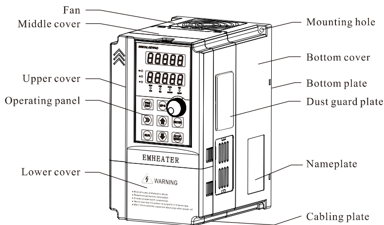
Diagram 2-2 Product appearance (With potentiometer)
