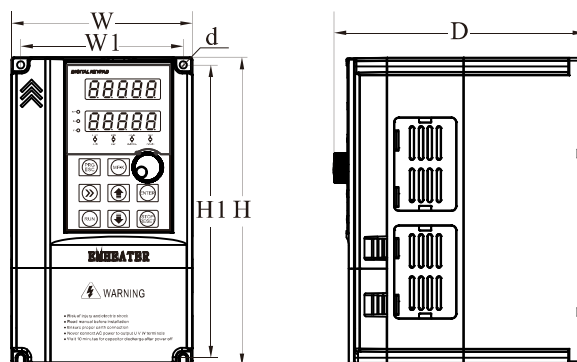
Diagram 2-3 Appearance and installing dimension of EM15 series (Plastic housing structure)
