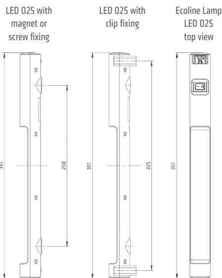
Side view magnet fixing
