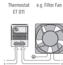
Wiring examples
