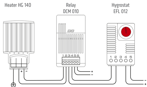
Wiring example
