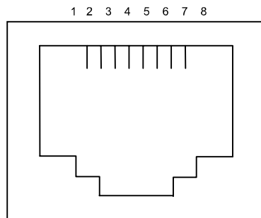
Figure 10 – Serial Port MJ1 RJ-45 Jack
