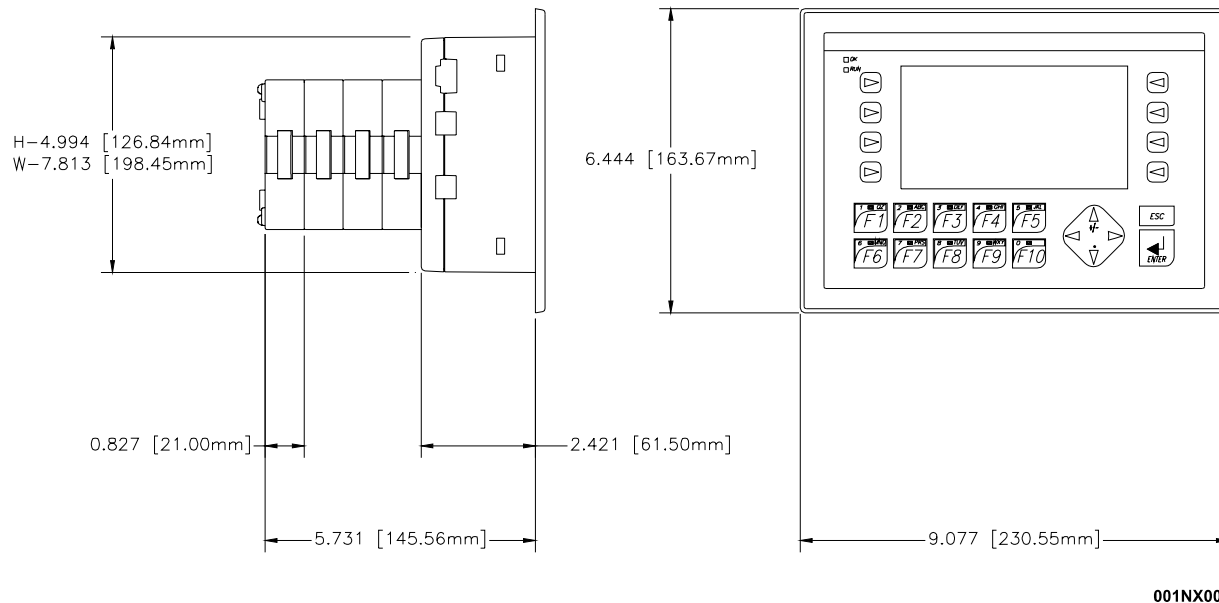
Figure 1 – Dimensions for the NX (NX25x is shown but dimensions apply to all NX Models) (Left figure shows side-view of NX with 4 SmartStack Modules attached.) (Right figure shows front view.)
